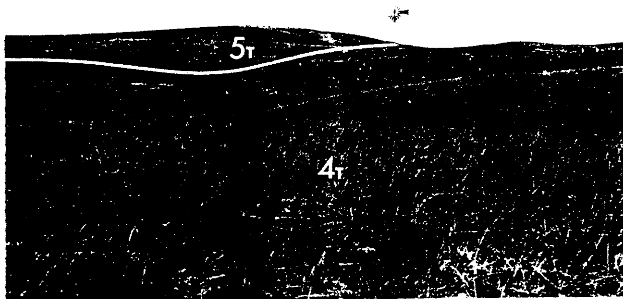
▲ FIGURE 9: This photograph was taken in the Brown Soil Zone of the prairies where the drouth hazard limits the top class of soil to Class 3C. The areas shown here have been further downgraded to Classes 4 and 5 because of topographic limitations.
